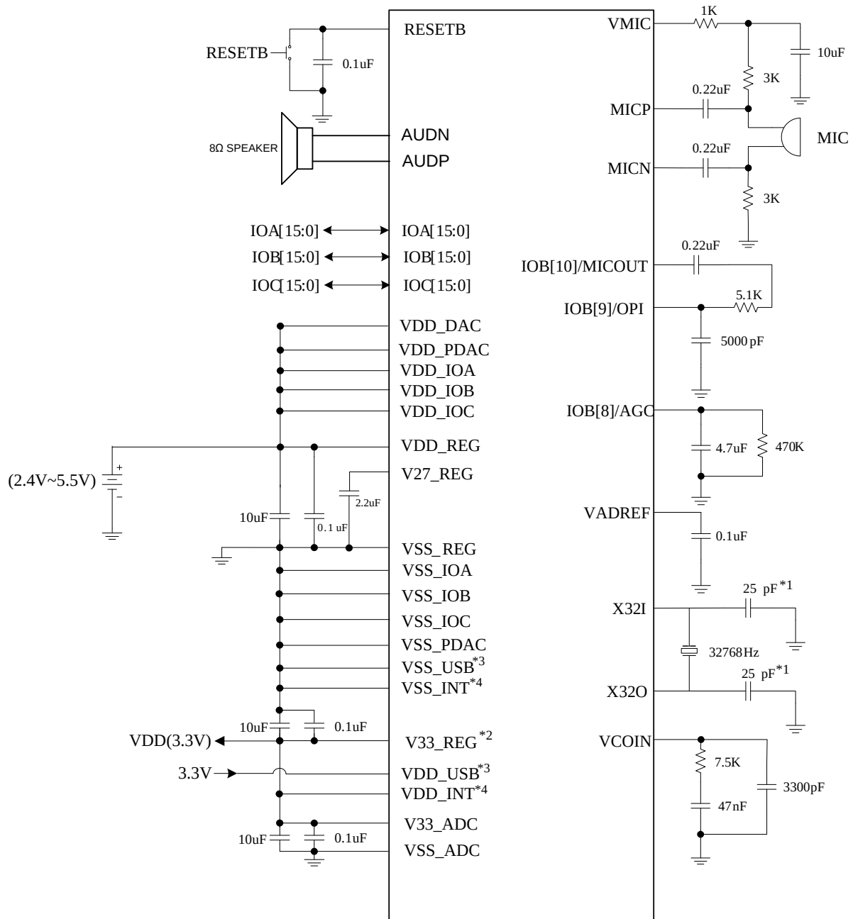
Application Circuit(MIC_IN )
